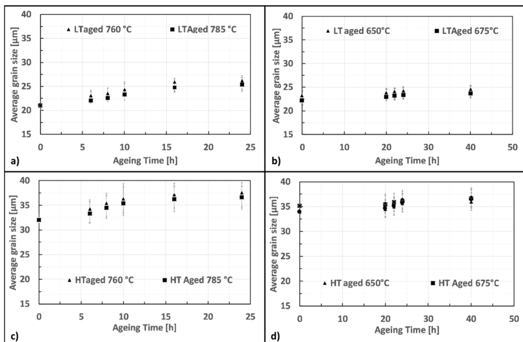
Figure 8. Effect of first and second aging on grain growth for LT and HT specimens: (a) first aging on LT, (b) second aging on LT, (c) first aging on HT and (d) second aging on HT.
