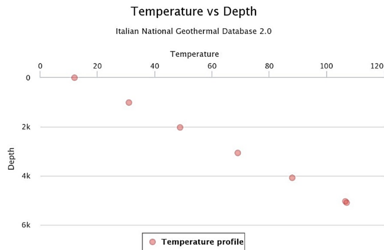
Figure 3. Temperature data visualisation for the Tempa Rossa 1D hydrocarbon well: Depth (m); Temperature (°C).
