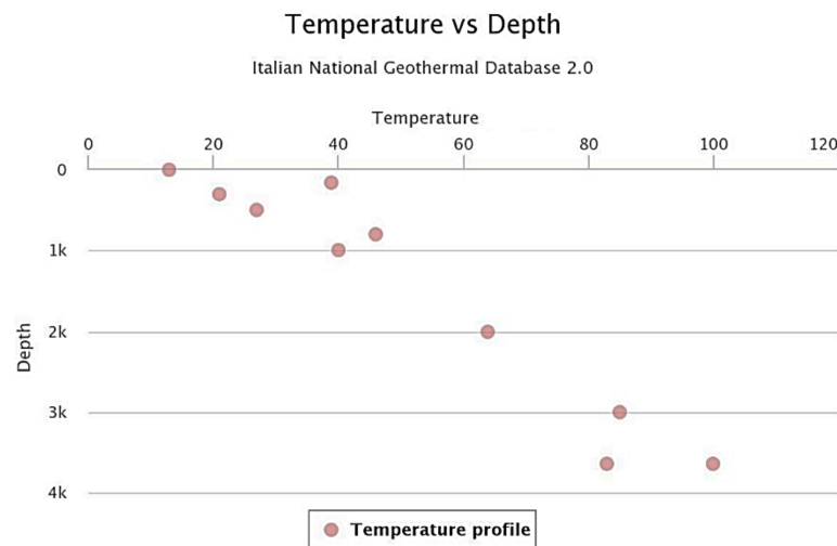
Figure 2. Temperature data visualisation for the Villafortuna 1 hydrocarbon well: Depth (m); Temperature (°C).
