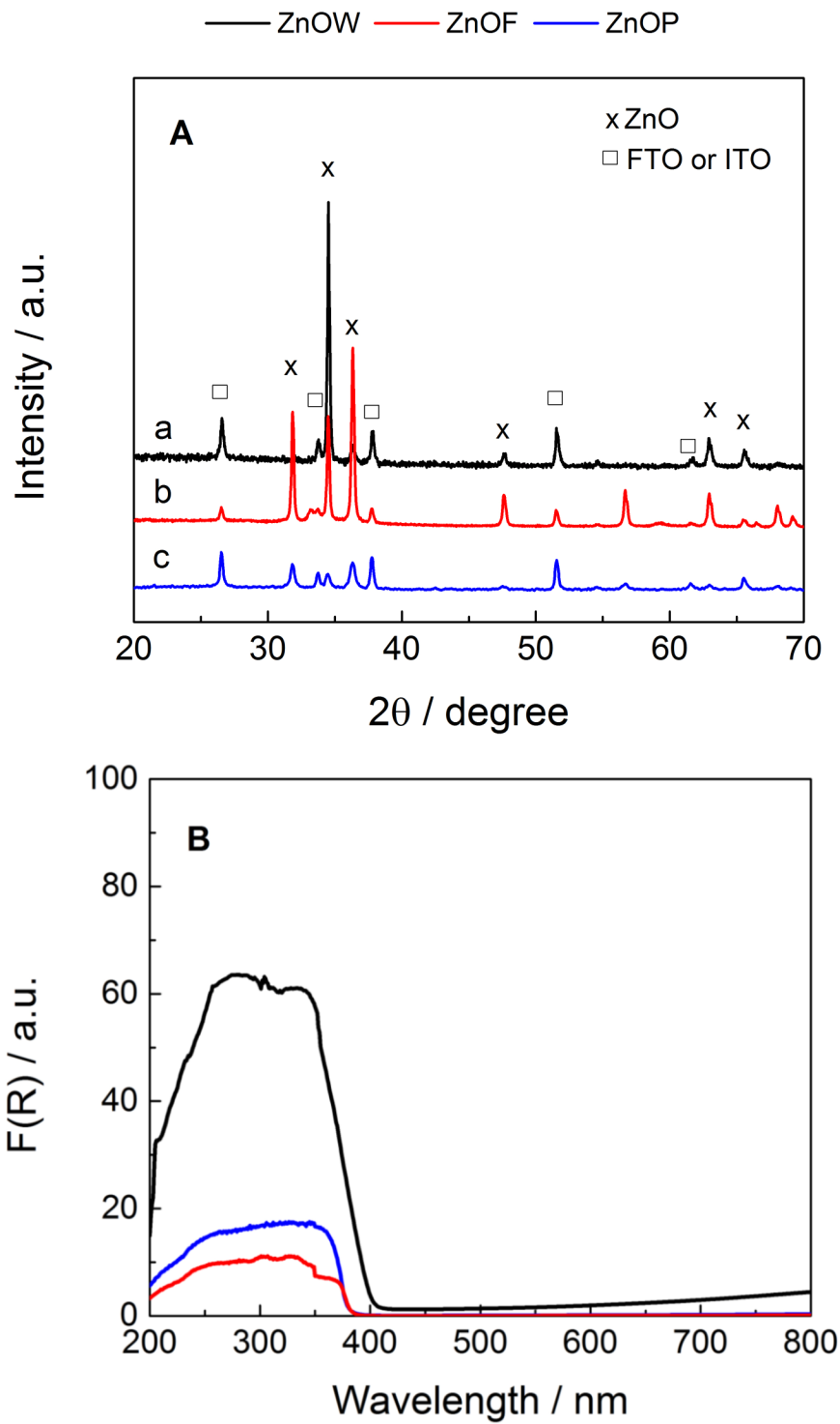
Figure 2. Physicochemical characterization of the different ZnO-based electrodes. A) XRD and B) UV-Vis reflectance F(R) spectra.
