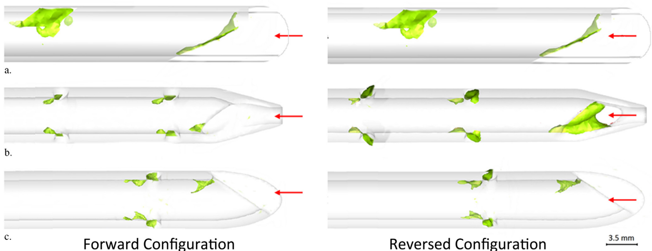
Figure 2. Flow separation regions for Palindrome ( a ), GlidePath ( b ), and VectorFlow ( c ) catheters in forward and reversed directions within the arterial lumen. The scale at the bottom of the image allows for quantitative analysis of the spatial extension of regions of disturbed flow inside the lumen; areas of flow separation appear in green. Red arrows indicate the main direction of flow.
