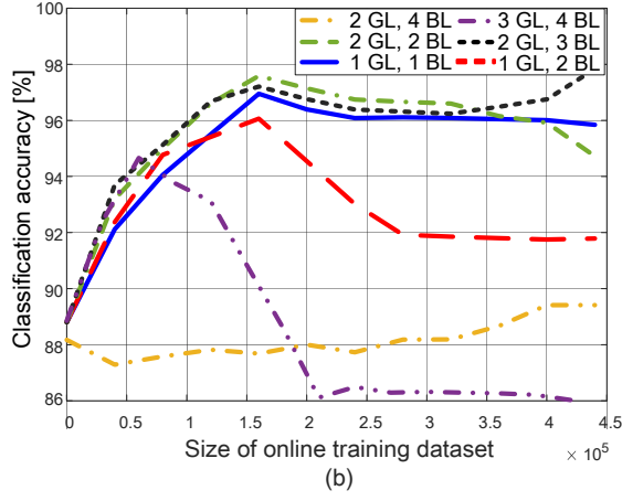
Fig. 10. Effect of the number and quality of labelers on the obtained classification accuracy, for a varying size of the online training set: (a) LS algorithm and (b) RLS. For the ego vehicle, the availability of 3 good-quality labelers and 4 bad-quality labelers is considered.
