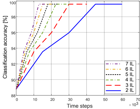
Fig. 11. Time of convergence for the IL selection, for different numbers of labelers.
