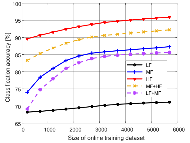
Fig. 13. Classification accuracy as a function of the size of the online training set, for different levels of freshness and M = 500 , while considering the data mode.
