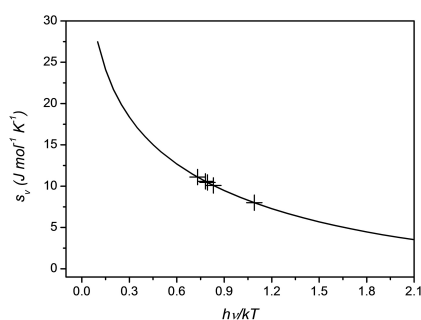
Figure 2. Plot of s_v as a function of the ratio \nu/T . The symbols correspond to the cases reported in Table 2.
