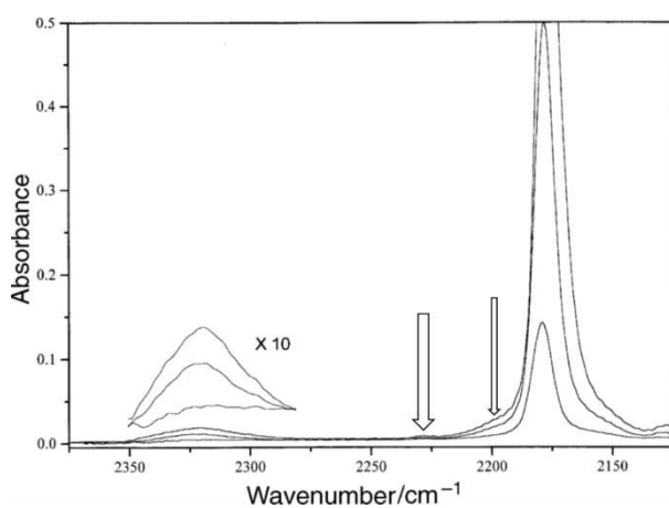
Figure 3. IR spectra of CO adsorbed on Na-ZSM-5. Arrows show combination bands between \nu(\text{C-O}) and \nu(\text{M-C}) modes.
