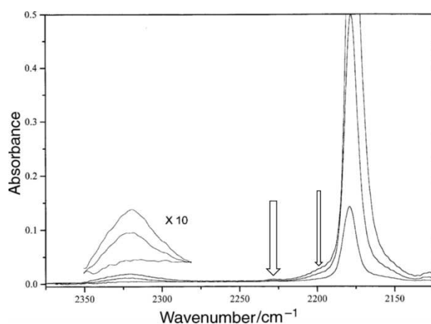
Figure 3. IR spectra of CO adsorbed on Na-ZSM-5. Arrows show combination bands between \nu(C-O) and \nu(M-C) modes.
