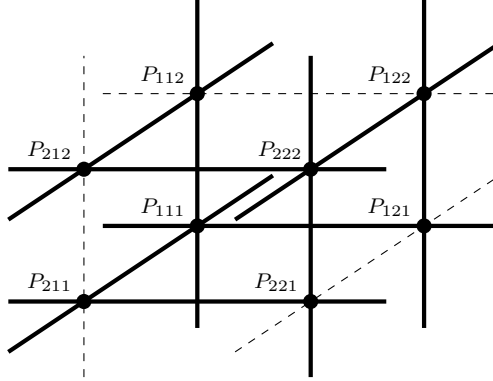
FIGURE 4. The variety of lines X (in bold).
