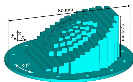
FIGURE 13. Perspective view of the SD 3D model. A ring of small holes at outer edges is for the screws to fix SD above RCA with cylindrical spacers.
