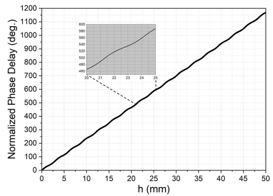
FIGURE 12. Normalized phase delay between two parallel planes separated by a fixed distance D = 50 mm. The space between the two planes is filled with dielectric material of \epsilon_r = 2.72 and varying height h .
