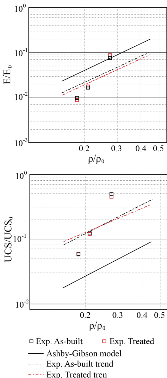
Fig. 7 Relative Young’s Modulus vs. relative density, and relative UCS vs. relative density.
