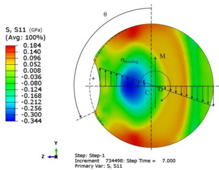
Figure 6. Normal impact: total stresses, 13.5^\circ \leq \theta \leq 22.5^\circ .
