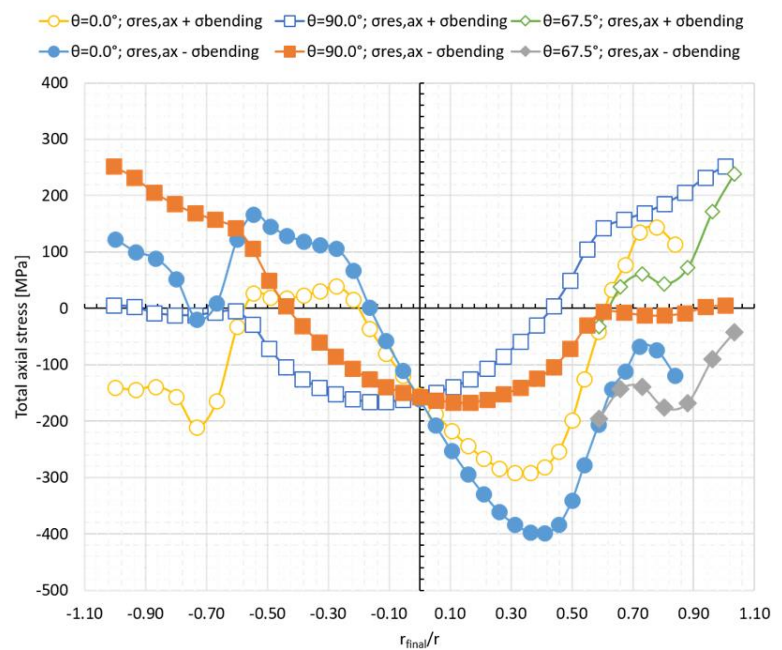
Figure 7. Normal impact: total stresses, \theta = 0.0^\circ, 67.5^\circ, 90.0^\circ .
