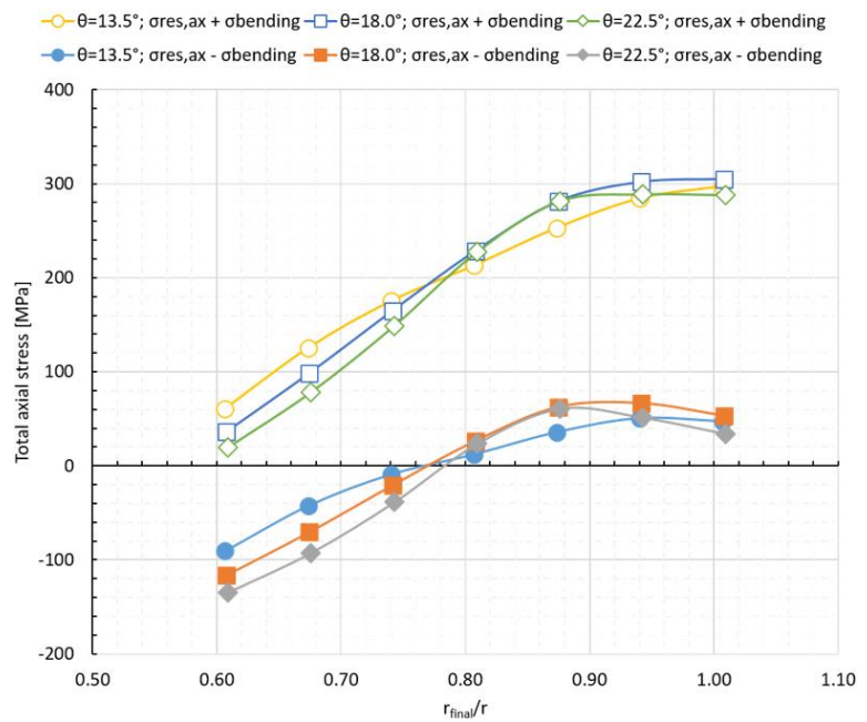
Figure 6. Normal impact: total stresses, 13.5^\circ \leq \theta \leq 22.5^\circ .
