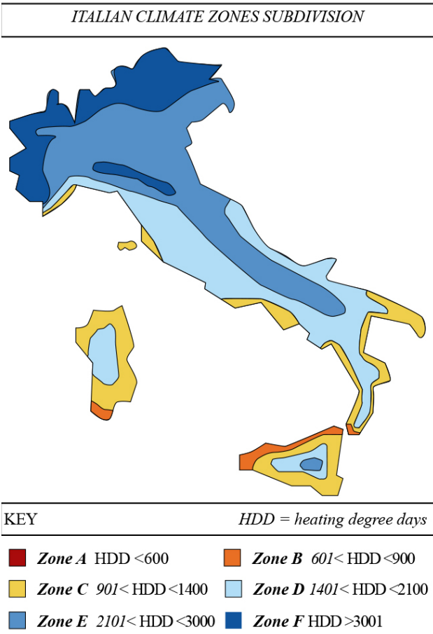
Figure 2. Italy Climate Zones. Zone E and Zone F were chosen in the building energy analysis.
