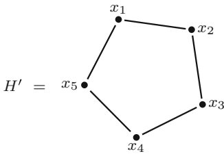
Fig. 4 The shadows of H on V' and V''
