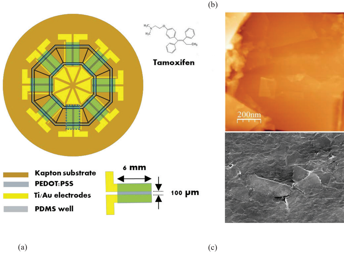
FIGURE 1. (a) OECD layout (inset: molecular structure of TAM); (b) AFM characterization of FLG on LDPE; (c) magnification of an exemplificative defect on the FLG surface by SEM analysis (Reprinted with permission from AIP Conference Proceedings 1599, 18 (2014). Copyright 2014 American Institute of Physics).
