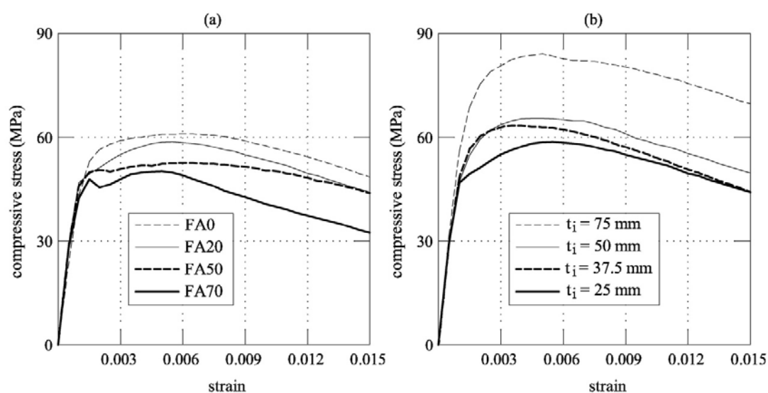
Figure 4. Stress-strain curves of the jacketed cylinders: (a) behaviour of different UHP-FRCC jackets having a constant of thickness t_j = 25 mm; (b) behaviour of the same UHP-FRCC jacket (FA20) having different thickness.
