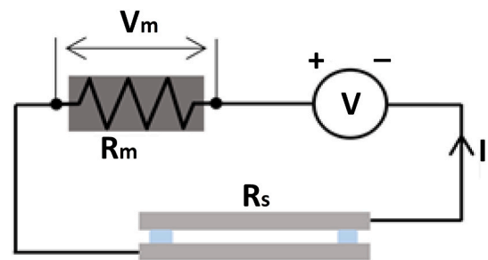
Fig. 1. Schematic of the measuring setup for electrical resistivity. The joint sample R_s is connected in series to a voltage generator V and a measuring resistance R_m .
