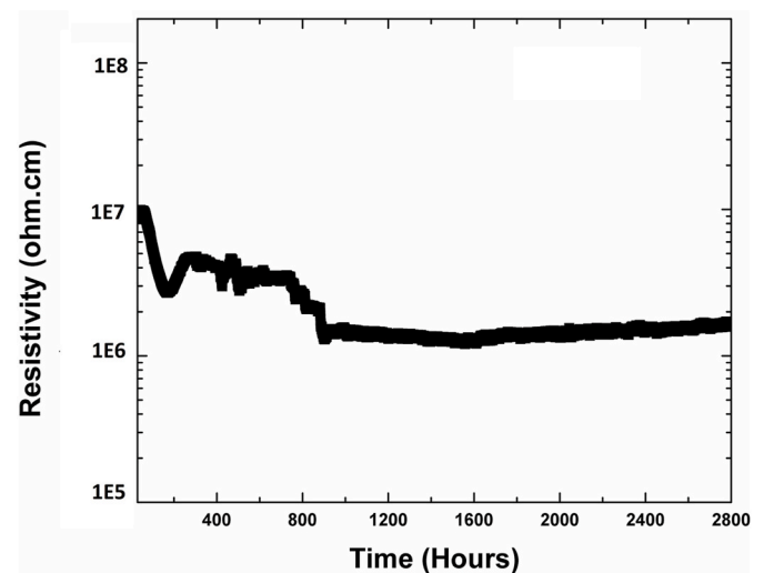
Fig. 2. Electrical resistivity of Crofer22APU/glass-ceramics/Crofer22APU joined samples for HJ4 glass-ceramics. These measurements were carried out at 850 °C with 1.6 V applied.
