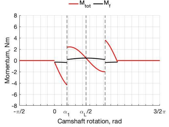
Figure 12. Total moment's trends for the simplification of a desmodromic system.
