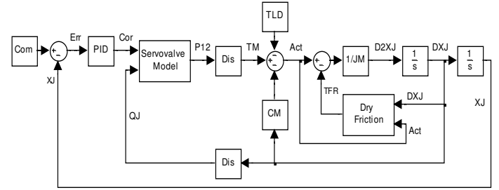
Figure 2: Theoretical actuator dynamics block diagram schematic
