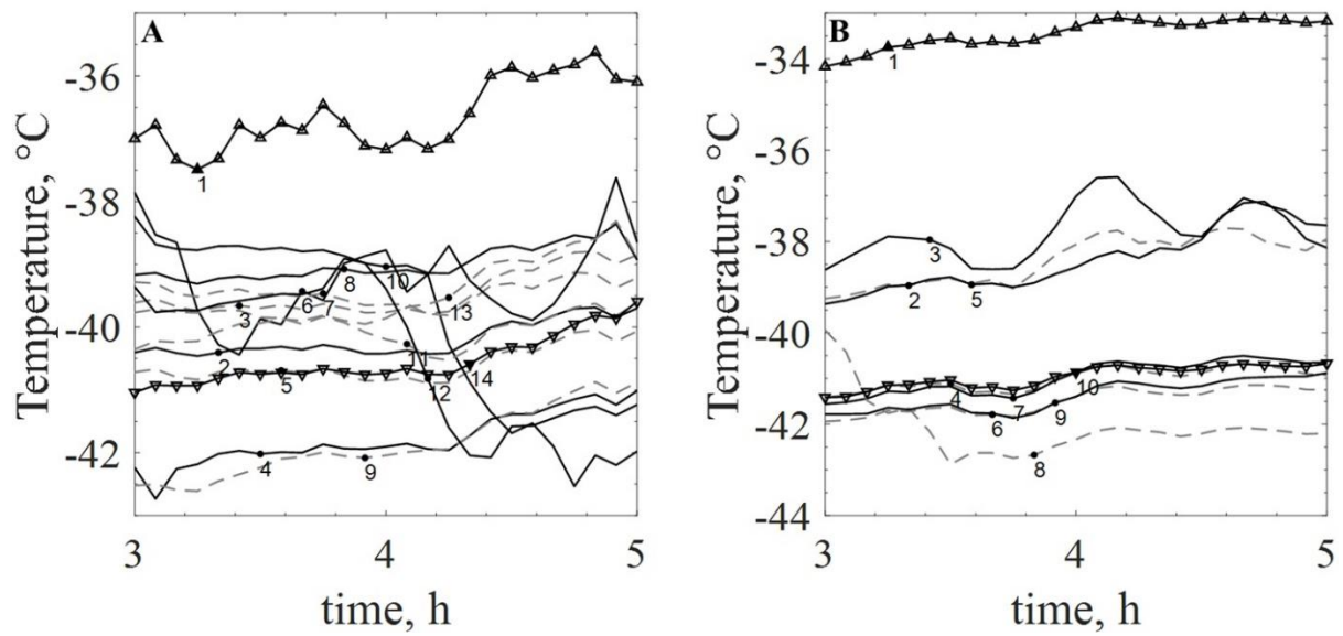
Figure A.8. IR bottom temperature profile by vial, in order from left to right, according to the thermal camera field of view. The first (leftmost) vial is represented with a line and triangle ( \blacktriangle ), the last (rightmost) vial is represented by a line and inverted triangle ( \blacktriangledown ). For all other vials, dashed lines represent ~central vials while continuous lines represent ~edge vials. (A) Shows results for 6R and (B) for 20R vials. Graph zoomed for the last 2 hours of primary drying.
