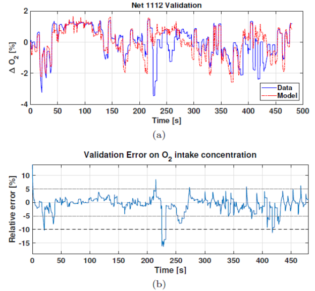
Figure 7. a) Network validation simulation. b) Network validation error.
