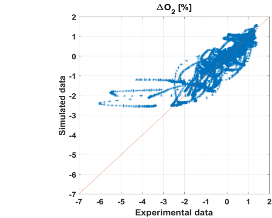
Figure 6. Simulated vs. experimental values of the intake O_2 concentration.
