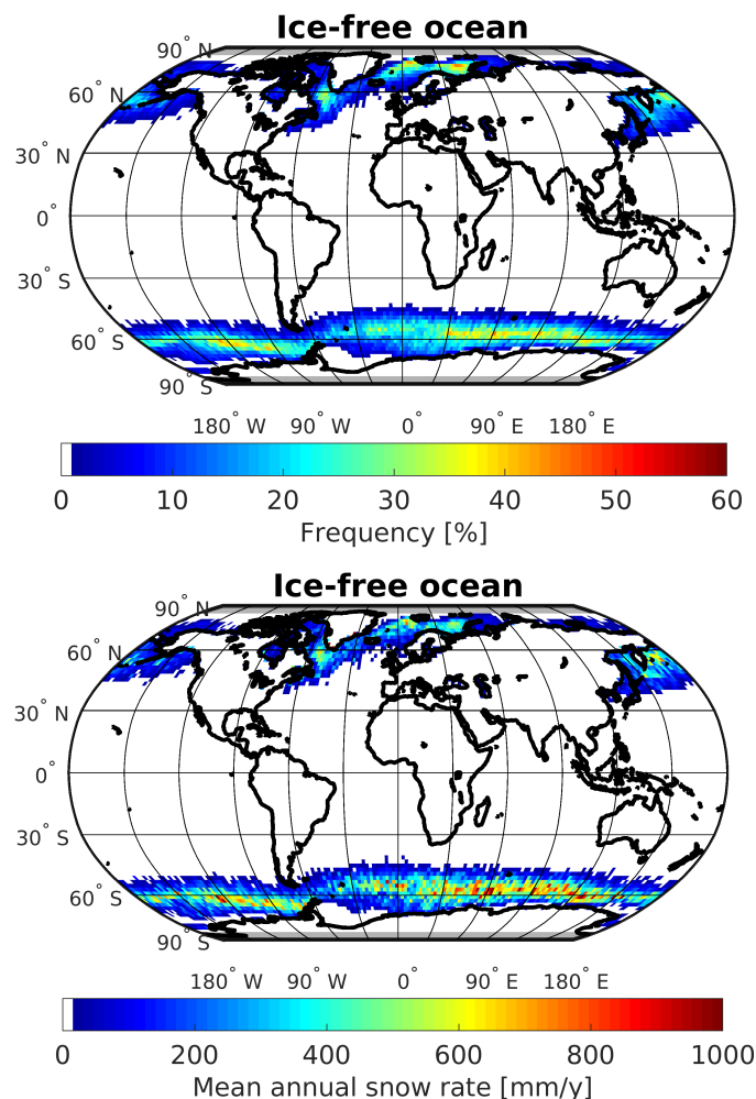
Figure 8. CloudSat derived snowfall occurrence (in %) ( top ) and mean annual snowfall rate ( bottom ) over ice-free ocean in 2° × 2° bins for the 2008 dataset. Snowfall occurrence is defined as the number of snowfall events over ice-free ocean divided by the total number of observations in each grid box.
