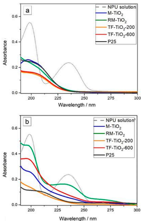
Figure 6. UV spectra (190–300 nm range) of the supernatant solutions concerning the photocatalytic degradation of NPU after 4 h illumination under UV light (a) and 1 Sun (b) in the presence of 1 \text{ g L}^{-1} P25 (black curve); M-TiO 2 sample (blue curve); RM-TiO 2 sample (green curve); TF-TiO 2 -200 sample (orange curve) and TF-TiO 2 -600 sample (red curve).
