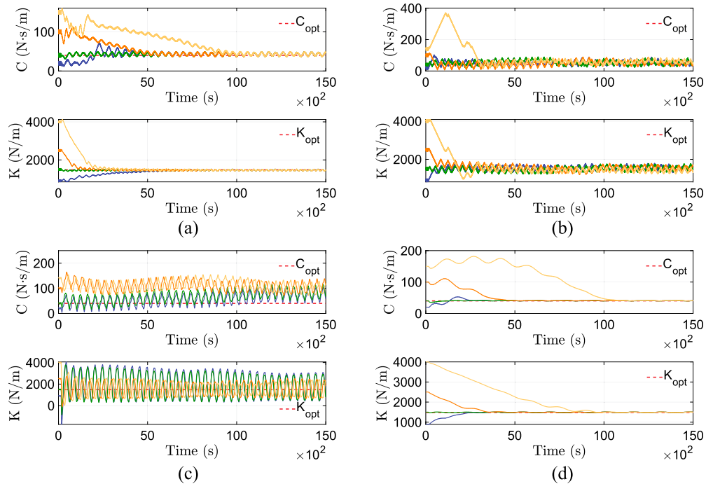
FIG. 24. Optimization of reactive and resistive coefficients, K and C , respectively, for the cylindrical buoy operating in the irregular sea state “Irreg.3” using (a) sliding mode, (b) relay, (c) LSQ, and (d) perturbation-based ES algorithms. The optimal K_{opt} = 1480 N/m and C_{opt} = 40 N s/m values are indicated by dashed lines in the plots.
