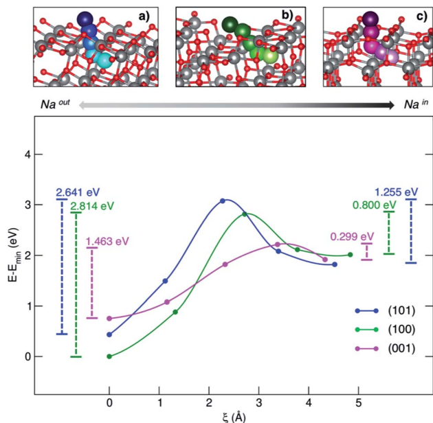
Fig. 3 MEP (top panel) and corresponding energetics (bottom panel) for the Na-migration through the (a) (101), (b) (100) and (c) (001) surfaces. Energy barriers calculated from eqn (4) and (5) for the out/in migration are reported, respectively, at the left- and right-hand sides of the graph.
