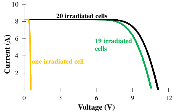
Fig. 6. I - V curves of a string with one, 19 and 20 cells under uniform irradiance condition.
