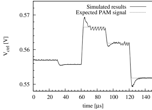
Fig. 6. VCO control voltage during a post-layout simulation (solid line), compared with the expected PAM signal (dotted line).
