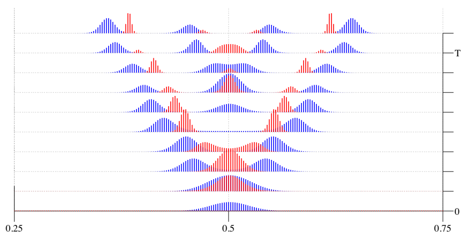
Figure 1. “Chase-and-escape” dynamics involving activated T cells and cancer cells without therapies. Evolution of n_C(t, u) (blue bars) and n_T(t, v) (red bars) at different times from t = 0 (bottom line) to t = T (top line). Clonal expansion leads to a rapid proliferation of those T cells that can effectively attack the antigens that are mostly expressed by the cancer cell population. The selective pressure exerted by activated T-cells causes, in turn, the selection of those cancer cells that are able to evade immune predation.
