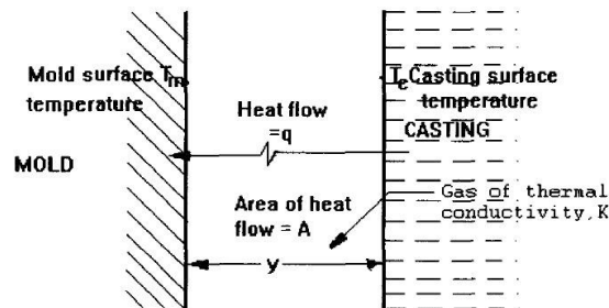
Fig. 4. Schematization of heat transfer mechanism, Krishnan and Sharma (1996).
