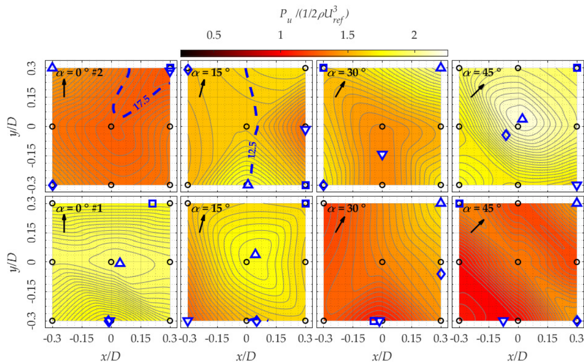
Figure 20. Wind Power density normalised against reference velocity, for configurations #1 (bottom row) and #2 (top row) and height z/D = 0.45 equivalent to 18 m in full scale. \nabla and \Delta indicate, respectively, the position of the lower and higher wind power density. Dashed blue contour lines show turbulence intensity I_u , with markers \diamond and \square , respectively, showing the position of lower and higher I_u .
