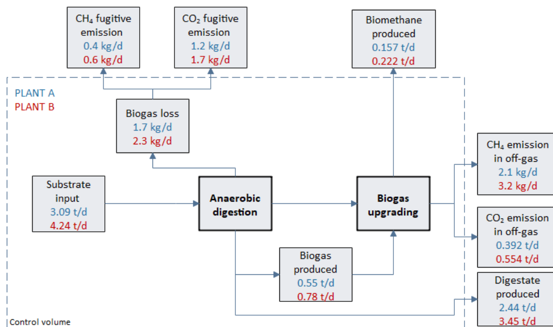
Figure 3. Mass balance of Plant A (in blue) and Plant B (in red).
