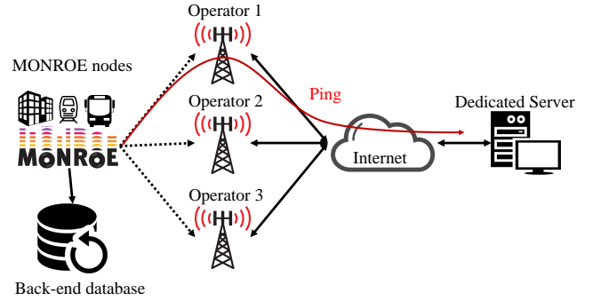
Fig. 1: The experimental setup for ping measurement in the MONROE platform.
