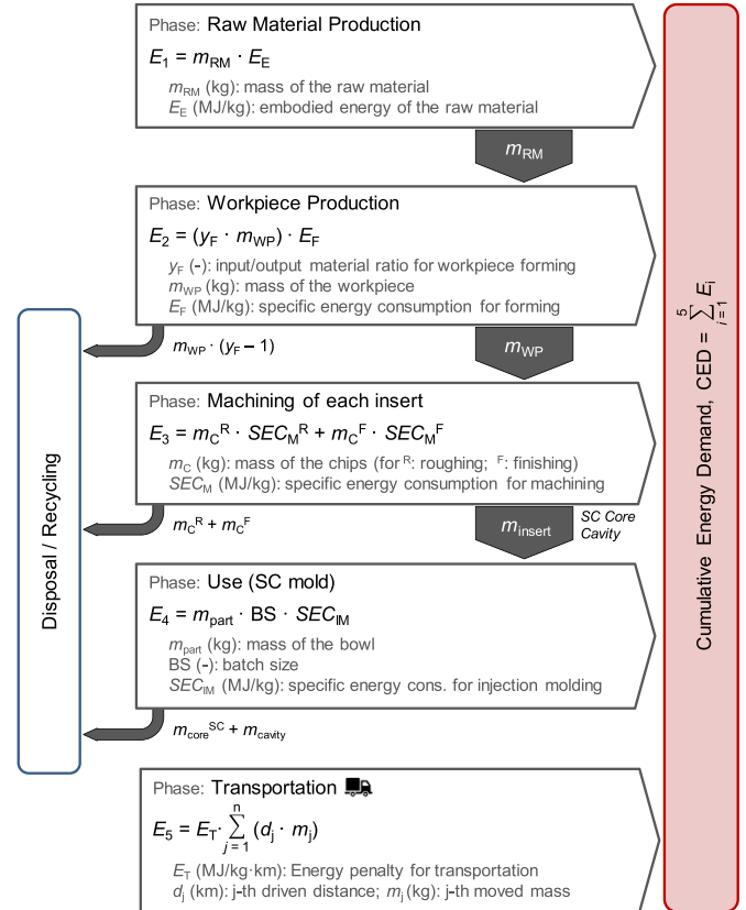
Fig. 2. Flowchart highlighting the machining approach.
