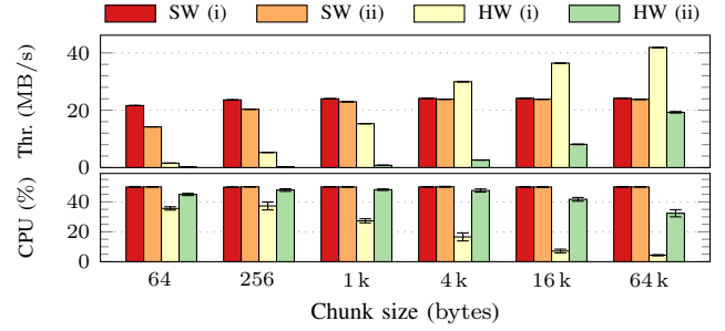
Fig. 8. Performance comparison between software and hardware implementations of AES-128-CBC, when encrypting multiple chunks of data within (i) the same and (ii) different cryptographic contexts.
