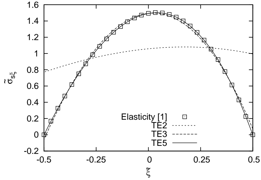
Figure 10: Dimensionless shear stress \tilde{\sigma}_{s\xi} at s = l/2 for a thick cantilever circular beam obtained by the proposed finite elements and an elasticity solution.
