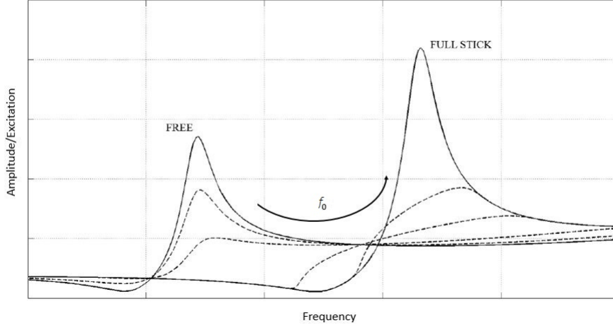
Figure 5: Stick-slip phenomenon in the frequency domain: an increase of the preload f_0 at the hooks has the effect of shifting the resonant frequency towards higher values, moving from the free to the full-stick configuration.
