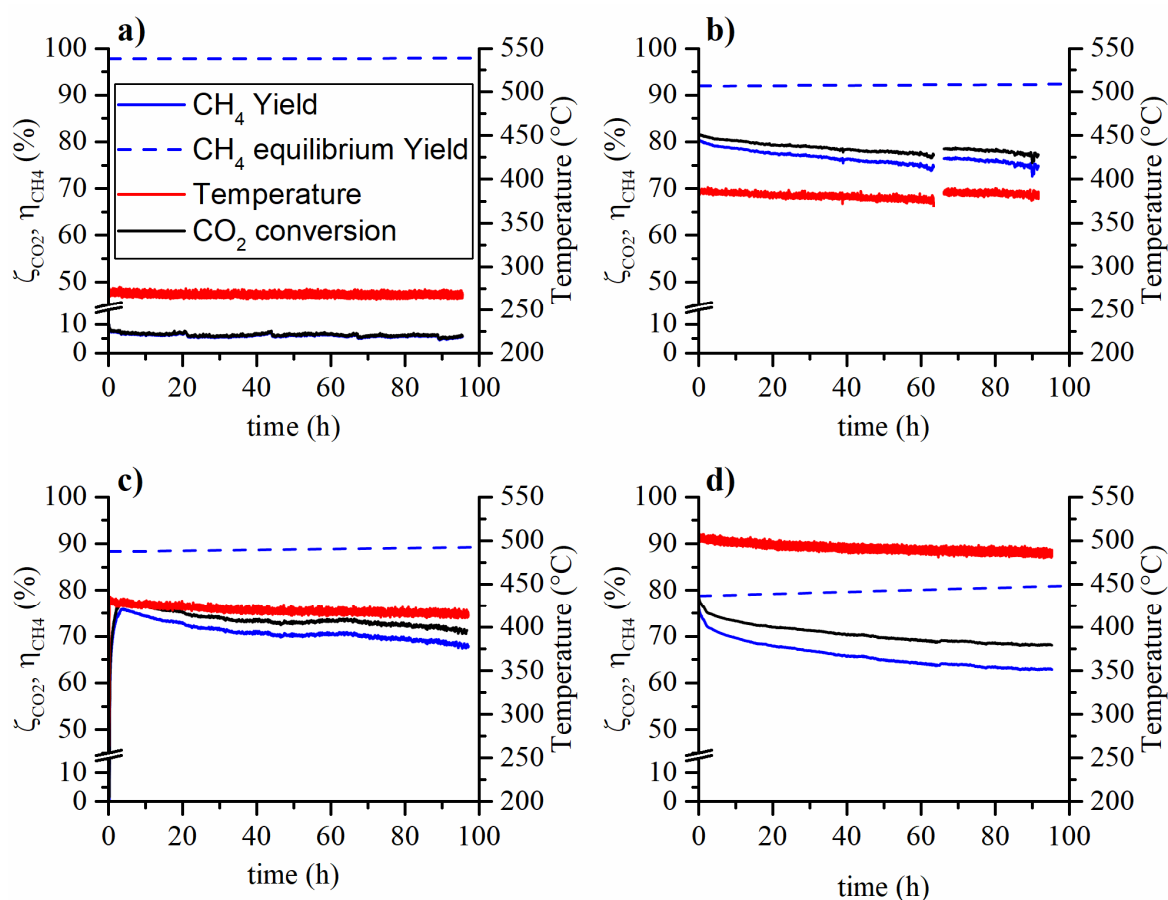
Figure 1. Aging tests at 5 bar, weight hourly space velocity (WHSV) = 150 ISTP g cat -1 h -1 , feed composition 16% CO 2 , 64% H 2 and 20% N 2 and (a) 270 °C, (b) 380 °C, (c) 425 °C and (d) 500 °C.
