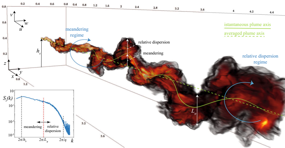
Fig. 1 Volume rendering of turbulent dispersion of a passive scalar released from a point source as simulated in a large-eddy simulation (2048 × 512 × 512 nodes for a domain of 6h_b \times h_b \times h_b , respectively in the along-wind, crosswind, and vertical directions). The blue arcs highlight two turbulent eddies of the same size. When the turbulent eddy is larger (smaller) than the plume size L_\phi , the eddy mostly contributes to meandering (relative dispersion). This is further highlighted in the turbulent energy spectrum S_t(k) (left-low panel); h_b and \eta are the boundary-layer height and the Kolmogorov microscale, respectively
