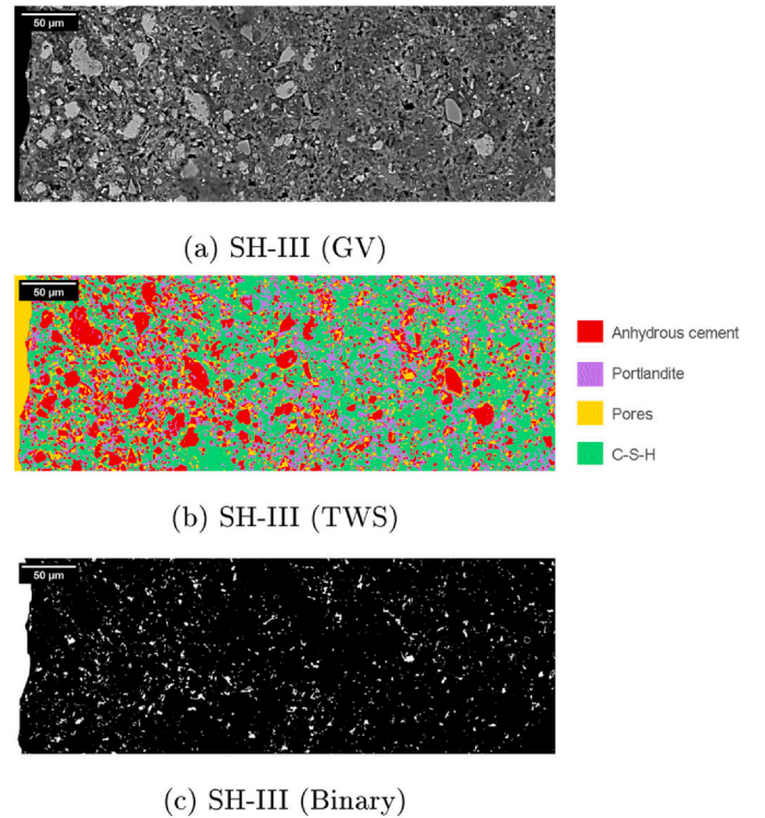
Fig. 5. BSE image of the interface zone of SH-III (PLA particle at the left) in Gray-Value a), after Trainable Weka Segmentation b) and after pore thresholding c).
