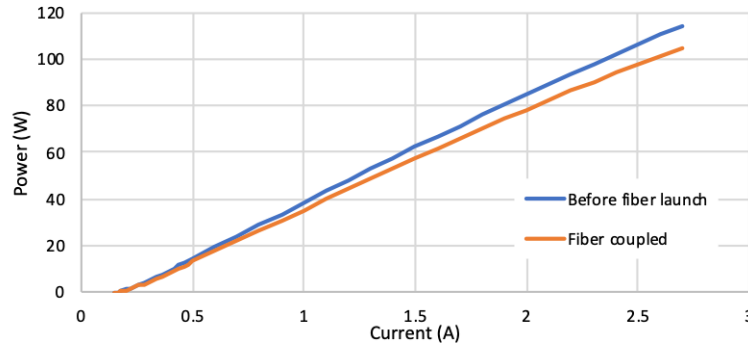
Figure 6. Final prototype output power against driving current, before and after the fiber coupling.
