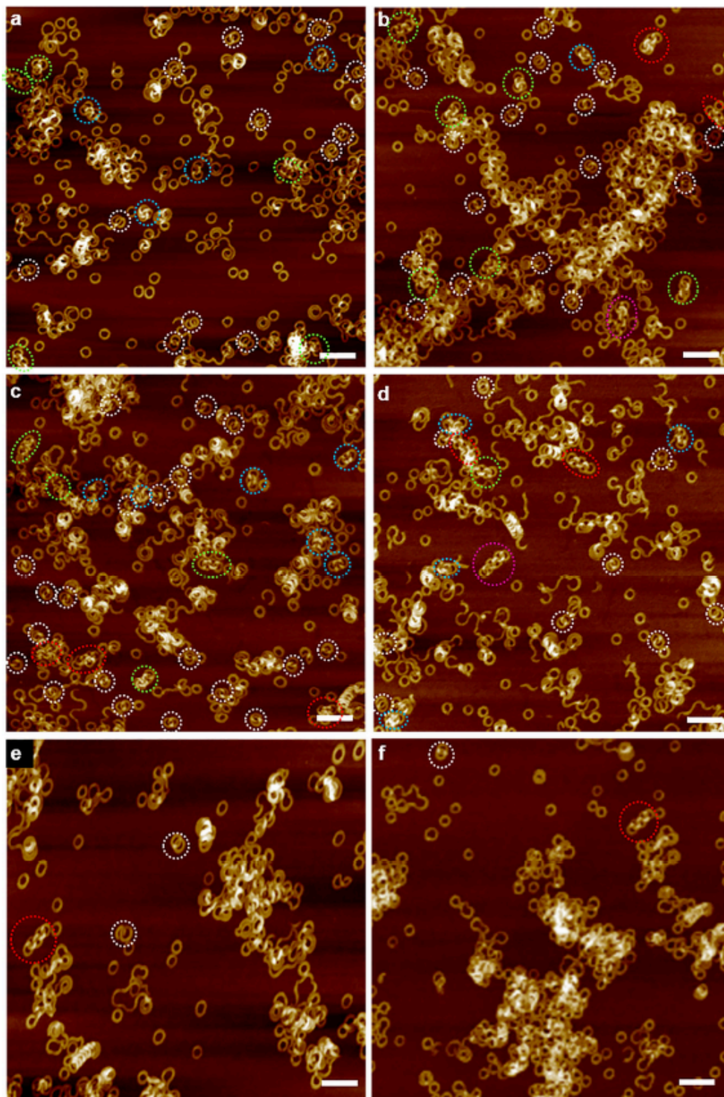
Extended Data Fig. 2 | AFM images of supramolecular polymers obtained in various n -alkanes by single-injection solvent mixing experiment. a–f , AFM images of supramolecular polymers prepared by injecting a 100 \mu\text{L} chloroform solution of 1 ( 1 \times 10^{-3} M) into 900 \mu\text{L} of n -hexane ( a ), n -heptane ( b ), n -octane ( c and d ), n -nonane ( e ), or n -decane ( f ) in one portion. Nano-[2], [3], [4], [5] and [6]catenanes are shown by dashed white, blue, green, red and pink circles, respectively. The samples were spin-coated onto a HOPG substrate at 293 K; scale bars = 100 nm.
