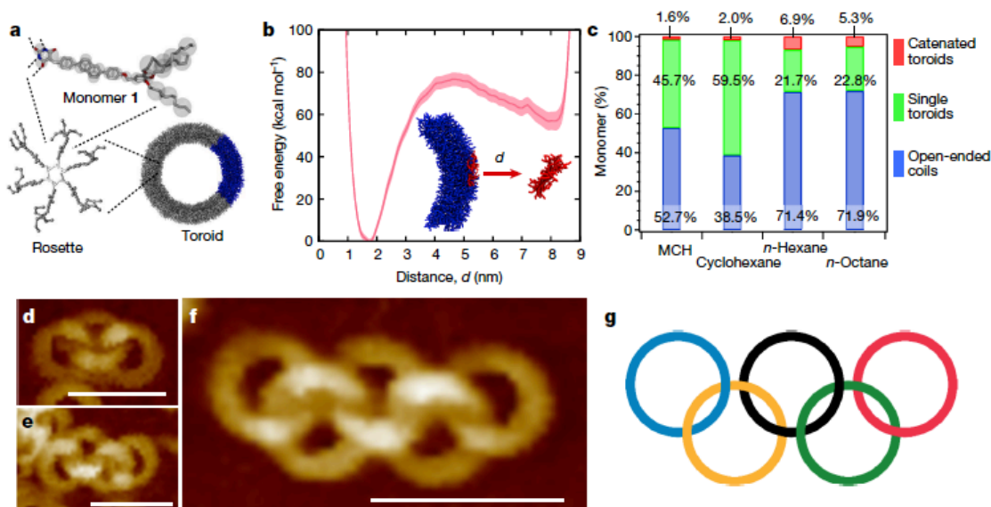
Figure 3 | Solvent dependence of the catenane yield. a , All atom (AA) and coarse-grained (CG) models of one monomer, one rosette (hexagonal assembly of six monomers) and one toroid of 1 used in the simulations. b , Free-energy profile for the interaction between one rosette trimer and the surface of the toroid (a portion of a full toroid composed of 50 rosettes) as a function of the distance ( d ) between the center of the toroid section (blue) and the center of the rosette trimer (red). c , Histogram showing the yield of catenanes (red bar), toroids (green bar), and random coils (blue bar) depending on the choice of poor solvent in single-injection solvent mixing experiment. d–f , AFM images of nano-[3]catenane ( d ), nano-[4]catenane ( e ), and nano-[5]catenane ( f ) obtained by injecting 100 \mu\text{L} of a chloroform solution of 1 ( 1 \times 10^{-3} M) into 900 \mu\text{L} of n -octane in one portion; scale bars = 50 nm. g , Symbol of the Olympic rings; reproduced with permission from the International Olympic Committee.
