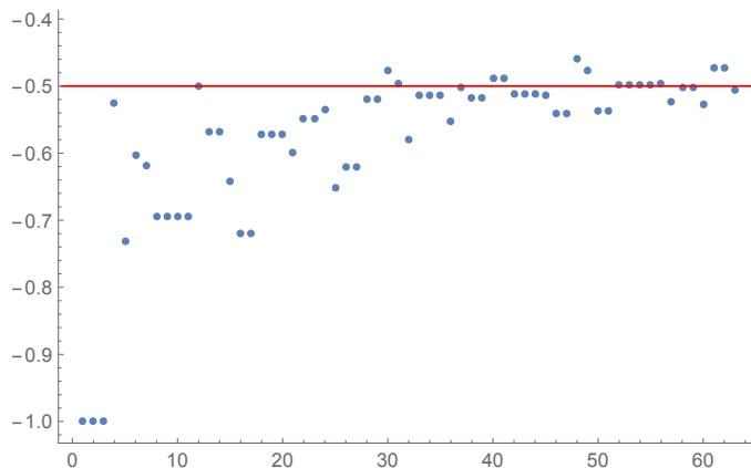
FIGURE 2. The first 64 values of \frac{\log \mathbf{m}_N}{\log L_N} , where L_N = \text{lcm}\{1, \dots, N\} = e^{N+o(N)} , plotted against the constant line -\frac{1}{2} . Les premières 64 valeurs de \frac{\log \mathbf{m}_N}{\log L_N} , où L_N = \text{lcm}\{1, \dots, N\} = e^{N+o(N)} , en comparaison avec la constante -\frac{1}{2} .
