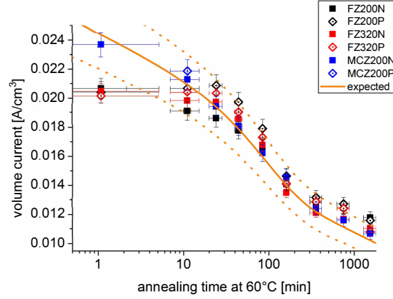
Figure 12. Volume current density as a function of annealing time at +60^\circ\text{C} shown for diodes irradiated with neutrons to \phi_{\text{eq}} = 4 \times 10^{14} \text{ cm}^{-2} . For comparison, the current density versus annealing time expected for this fluence based on a parameterization and parameters obtained by previous fits to data [1, 3] is depicted by a solid line. The corresponding uncertainty, shown as dashed lines, is due to the uncertainty in the fluence, estimated to be about 10%.
