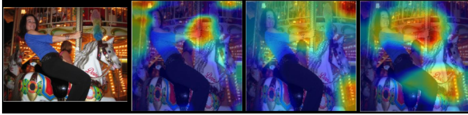
Fig. 3. Visual comparison of the predictions made by the three models in T1. The overlapping heatmap has been produced by the GradCAM algorithm. This is image was selected by the majority of the participants from the Suggestion view as an example of high confidence and high agreement classification. All the models are focusing on similar visual features to classify the frame. Best seen in RGB; consider brighter areas of the frames in case of gray scale visualization.
