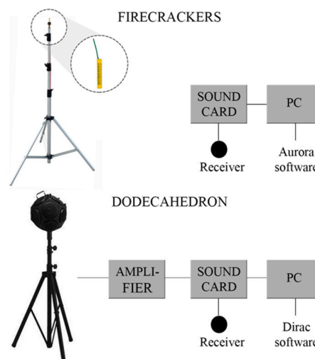
Figure 3. Measurement chains for the two source types—firecrackers ( top ) and dodecahedron ( bottom ).
