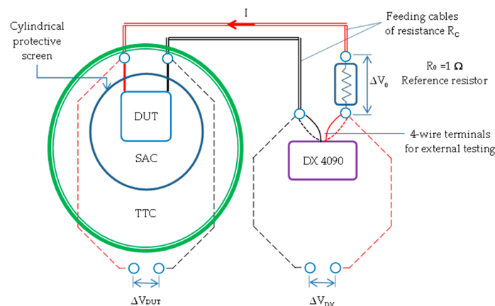
Figure 1. Scheme of the experimental arrangement. DX 4090 is the z-meter, TTC is the Thermo-Static Test Chamber, SAC is the Still Air Chamber, and DUT is the Device Under Test. Solid and double red and black lines are the feeding cables, while the dashed ones represent the signal wires.
