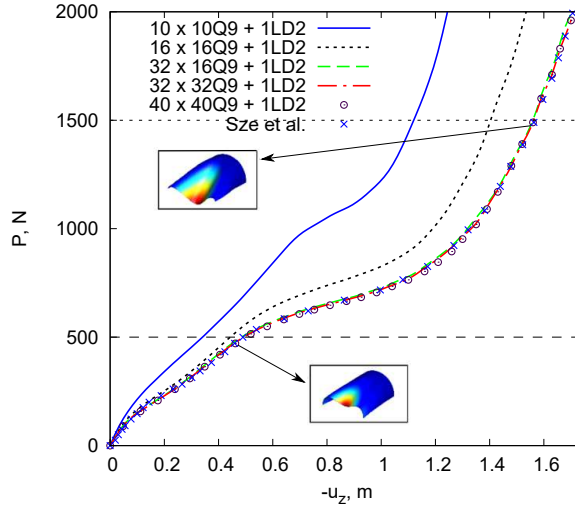
Fig. 5. Convergence study of nonlinear response curves for the isotropic pinched cylindrical shell. Comparison of different in-plane mesh approximations
