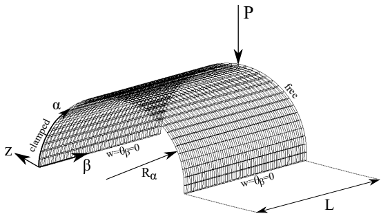
Fig. 3. Geometric properties, boundary and loading conditions of the pinched cylindrical shell
