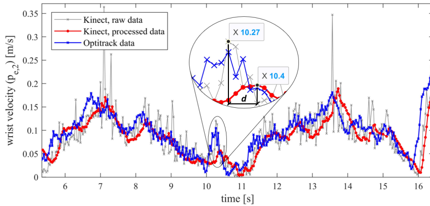
Fig. 5. Wrist absolute velocity module. A comparison between OptiTrack down-sampled data with raw and processed Kinect data. Test with linear-trajectory movements.
