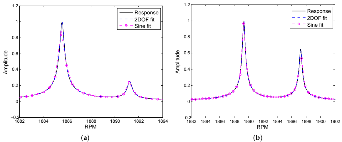
Figure 7. Comparison of non-dimensional amplitudes obtained by different fitting methods for EO = 5 and \zeta_{1,2} = 0.0001 , (a) SD = 0.05, (b) SD = 0.10.
