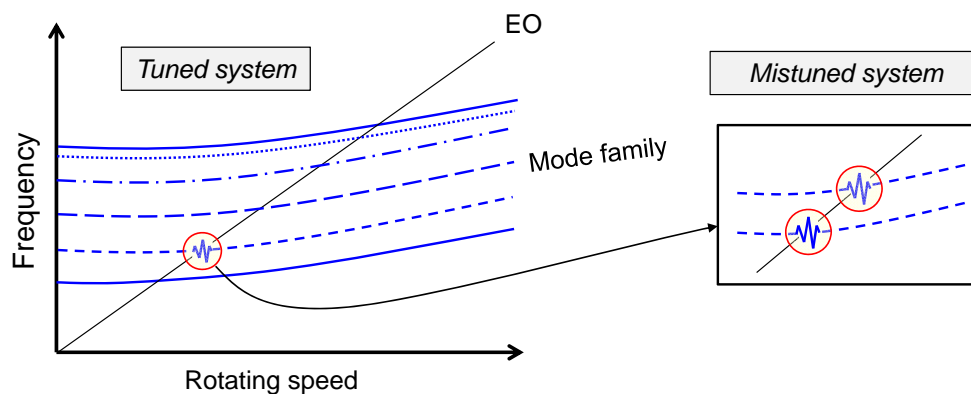
Figure 4. Splitting frequency in a mistuned system.
