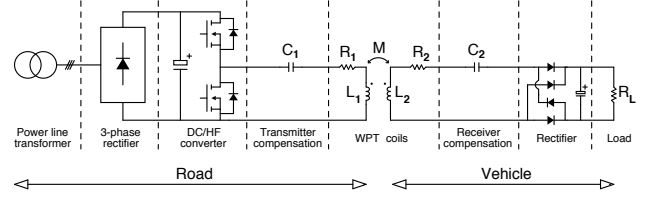
Fig. 3: Architecture of the CWD system.
