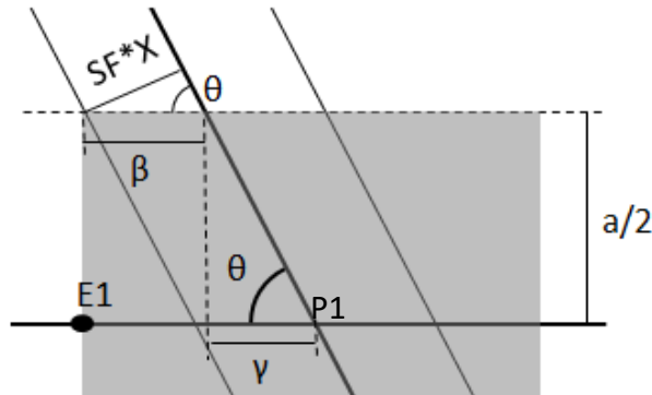
Fig. 2. Geometrical parameters of virtual segregated area
