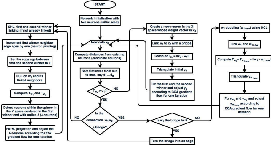
Fig. 1. The GCCA flowchart
